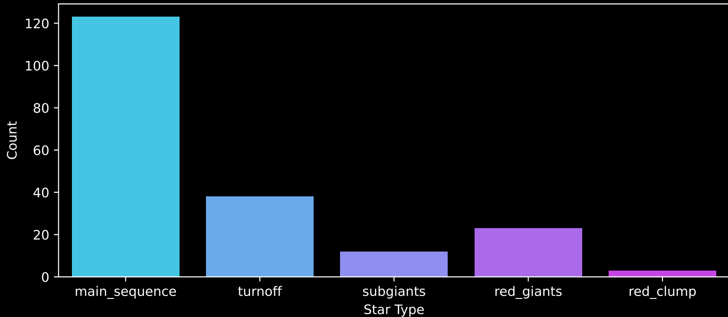
APOGEE DR17 Field: [046-47-O] Count plot of Star Type
