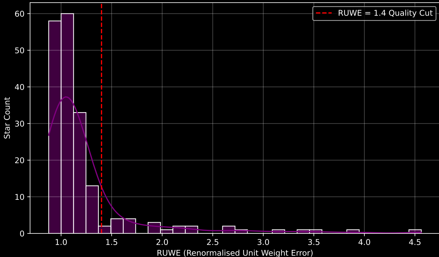
GAPOGEE DR17 Field [046-47-O] RUWE Distribution (n= 190)
