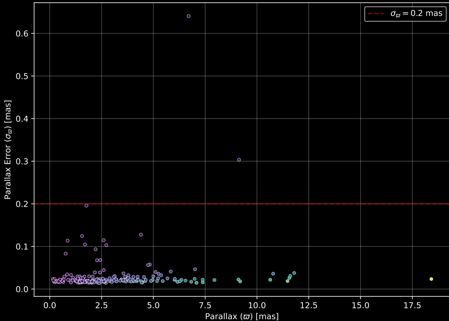
APOGEE DR17 Field: [046-47-O] Parallax Quality (n= 199)
