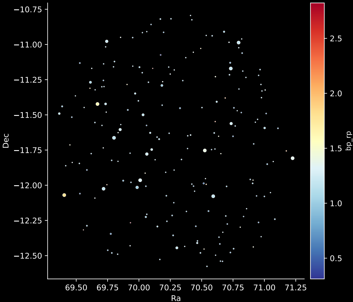
APOGEE DR17 Field: [046-47-O] Stars: 199
