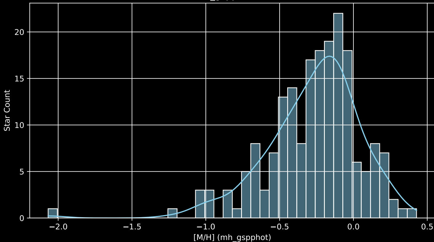
APOGEE DR17 Field: [046-47-O [M/H] (mh_gspphot) (n= 194)
