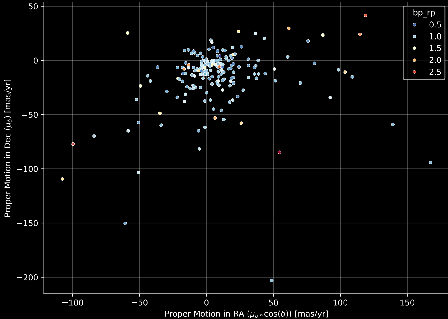
APOGEE DR17 Field: [046-47-O] Proper Motion Diagram (n= 199)
